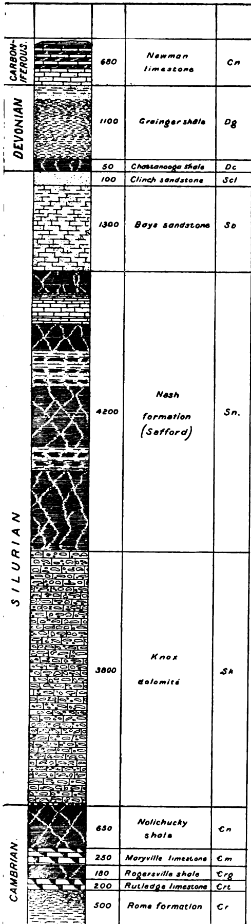
London sheet; stratigraphy of the syncline northwest of Chilhowee mountain.
